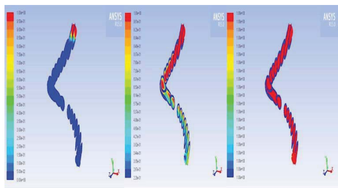
Fig 9 Distribution of volume fraction of liquid nitrogen on isosurfaces created at different positions of a helically coiled transfer line at different intervals of time.
