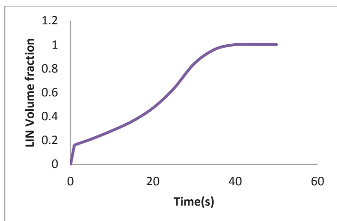
Fig 8 Variation of liquid nitrogen volume fraction with time at the solid fluid interface of a helically coiled transfer line
