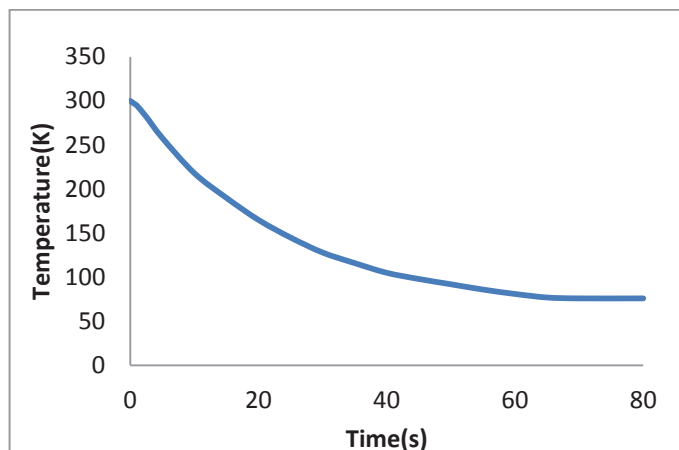
Fig 4 Variation of temperature with time at the solid fluid interface of a straight transfer line
