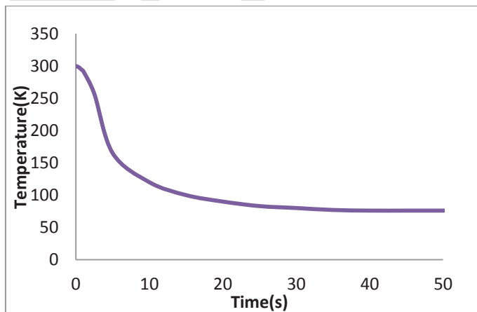
Fig 7 Variation of temperature with time at the solid fluid interface of a helically coiled transfer line
